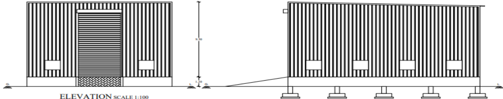
ELEVATION SCALE 1:100
