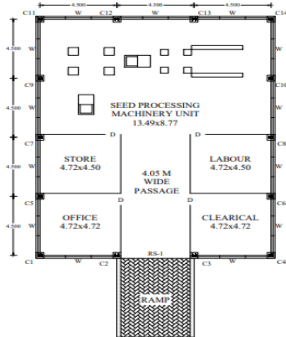
PLAN SCALE 1:100
